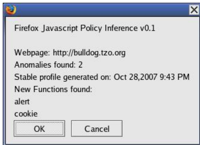
Figure 5.8: WebCal anomalies
