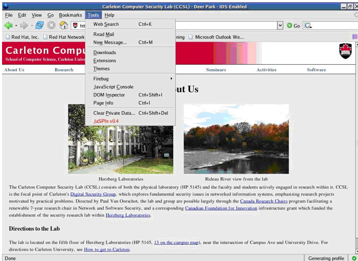
Figure 4.3: JaSPIn extension
