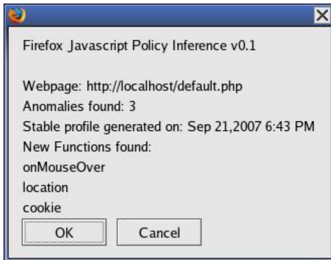
Figure 5.6: JaSPIn is able to detect the documented XSS exploit on phpBB
