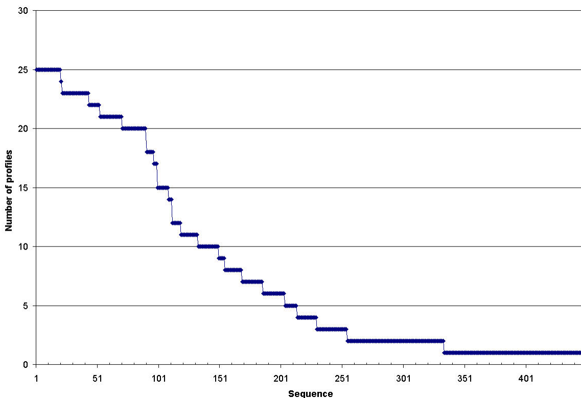
Figure 5.3: This graph shows the number of profiles containing each sequence of length 6 sorted by frequency. There are 25 profiles created from different visits to http://www.yahoo.com , which in total contain 449 unique sequences.
