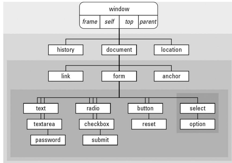
Figure 2.1: JavaScript object hierarchy
