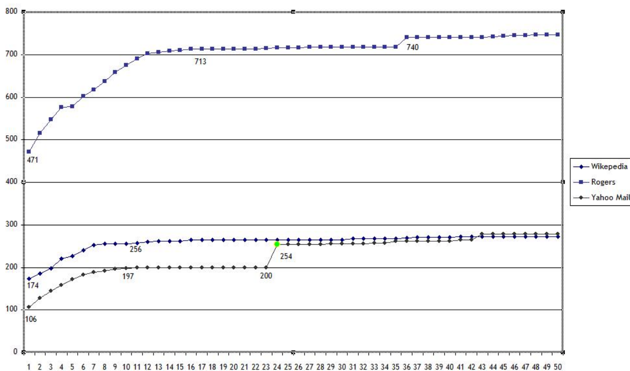
Figure 5.1: This graph shows the number of sequences observed per web site over a period of 50 visits. There are varying number of sequences in each web site’s profile. The first visit generates a brand new policy, and the next few visits stabilize that policy.
